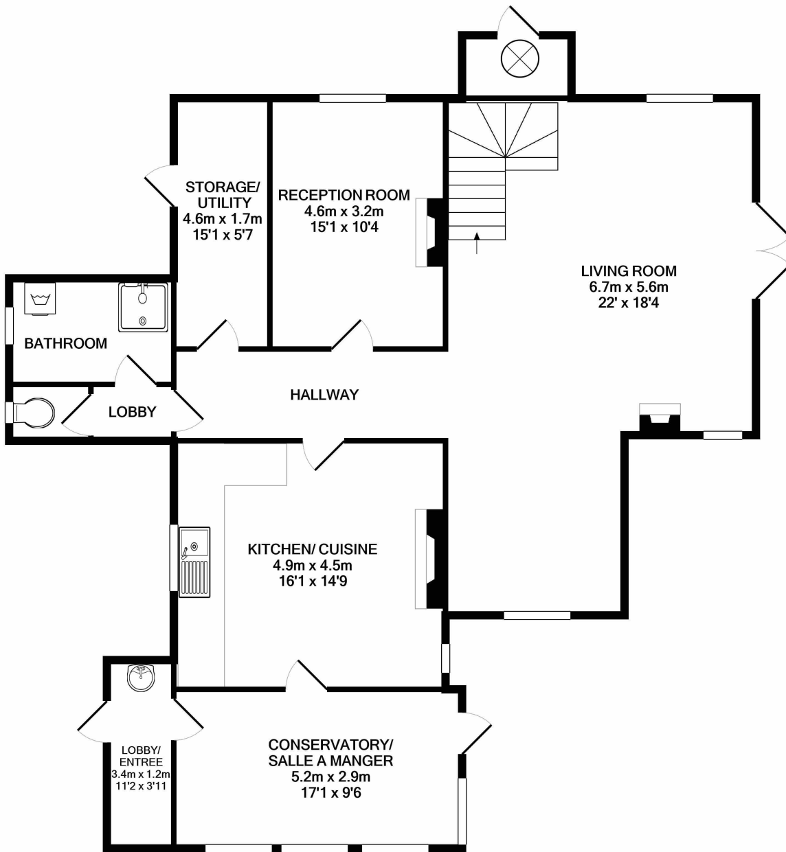
GROUND FLOOR
